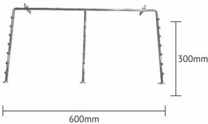
E-TYPE CHANNEL HANGER STAND DC-19
