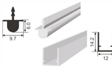
CABINET SLIDING CHANNEL 'A' DC-255
