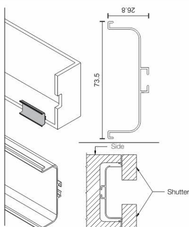
C-GOLA PROFILE DC-1111
