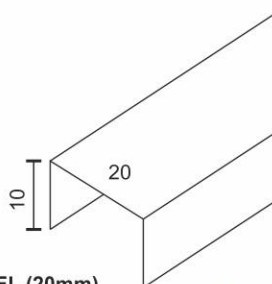
U-TYPE CHANNEL (20mm) DC-1151
