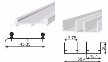
WARDROBE SLIDING CHANNEL (Double Track) DC-246
