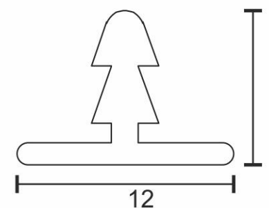
INLAY DECORATION PROFILE (12MM) DC-1106
