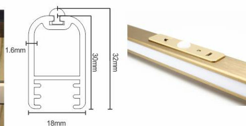
LED WARDROBE PIPE WITH INBUILT BATTERY DC-1105
