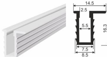
HI-TECH CABINET SLIDING CHANNEL DC-248
