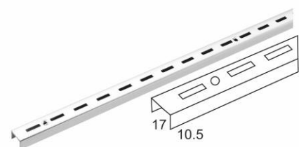
BRACKET CHANNEL (Single Slot Broad) DC-04
